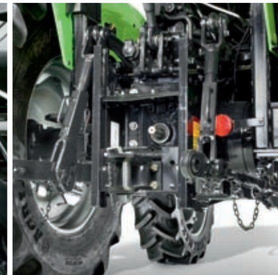
Simple but powerful at the same time: The hydraulic system with mechanical powerlift control.
