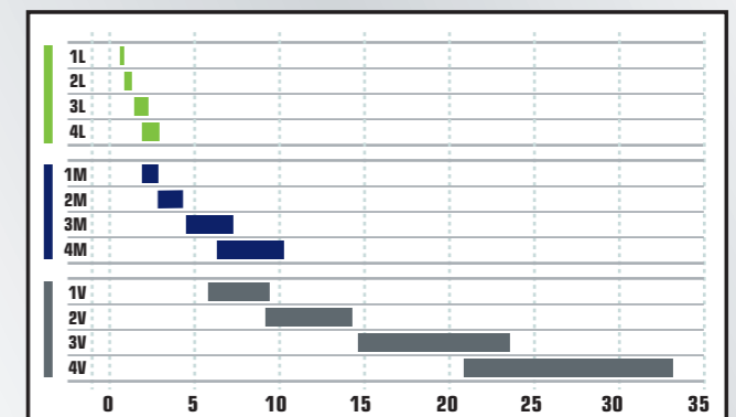
Perfectly graduated for every job: The Synchronsplit transmission.
